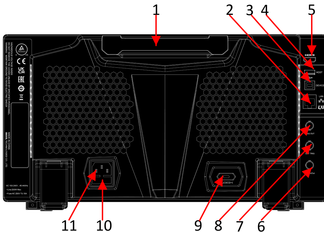
Figure 6.2 Rear Panel
