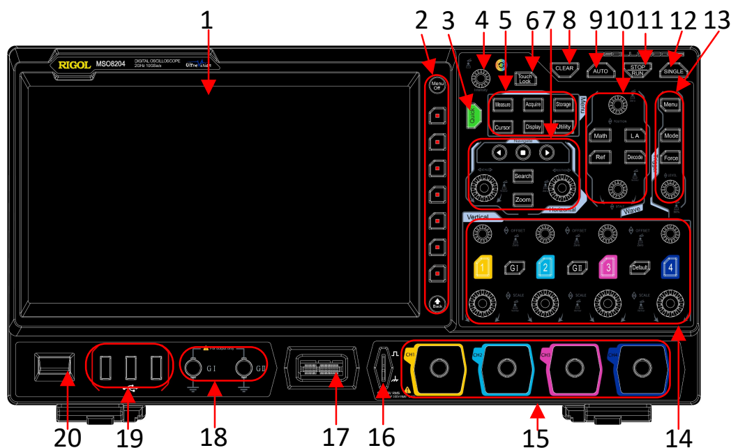
Figure 6.1 Front Panel
