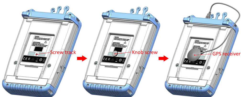
Figure 3-11: Location of GPS receiver
