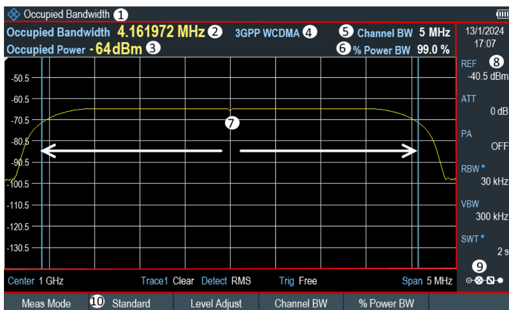
Figure 6-2: Screen layout for the occupied bandwidth
