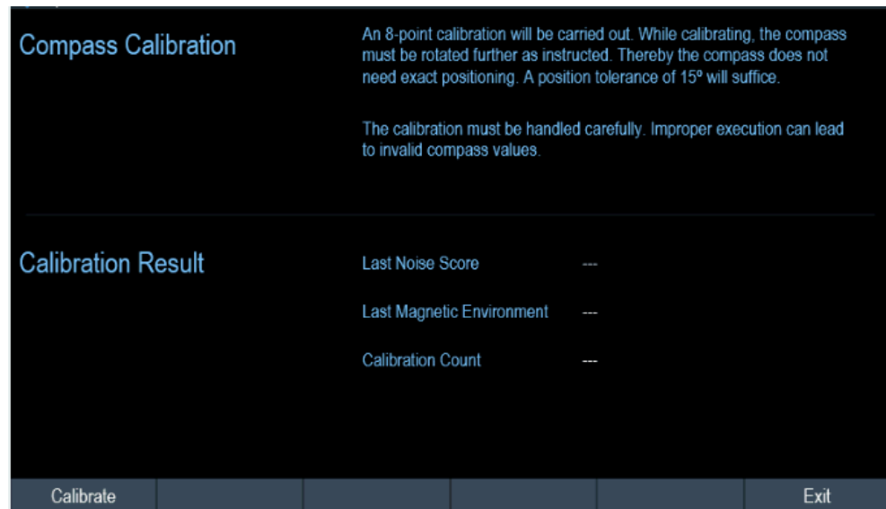
Figure 3-10: Display of compass calibration instruction and last calibrated result
