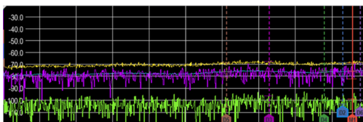
Figure 3-6: An example of the measurement trace window with four traces
